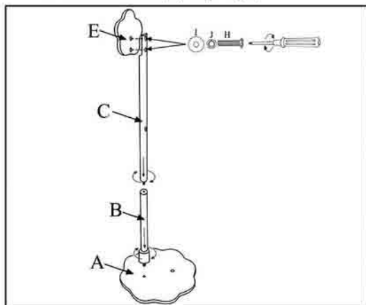
Fig. 1 Attach Mama pole (B, C) to Base (A) and Mama flower (E) to pole (C)
